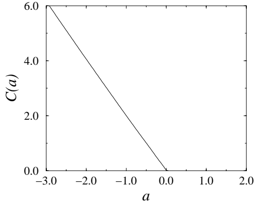
Fig. 2. Amplitude C(a) for the TM1 sequence with \kappa = 1/2 deduced from FSS at criticality with L_n = 6^n , n = 1, 7 . The surface transition is continuous for a < 0 and first-order for a > 0 .
