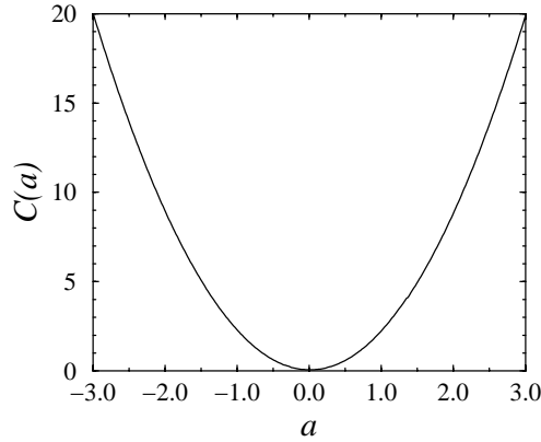
Fig. 6. Amplitude C(a) for the TM2 sequence with \kappa = \omega deduced from FSS at criticality with L_n = 6^n , n = 1, 7 . The surface magnetization vanishes continuously with a parabolic amplitude in the stretched exponential.
