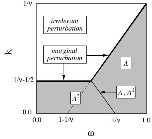
Fig. 13. Relevance-irrelevance of aperiodic extended surface perturbations in a system with bulk correlation length exponent \nu . The perturbation is relevant in the shaded region. The order of the dominant perturbation terms is indicated, assuming that off-diagonal terms do not contribute.
