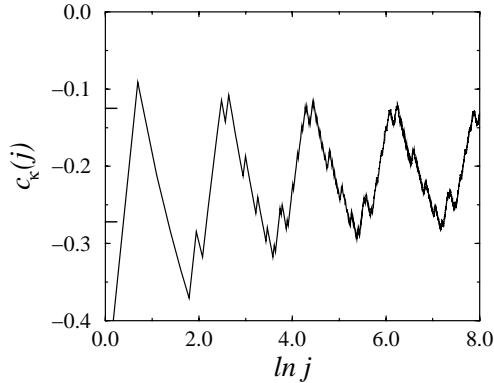
Fig. 3. Amplitude c_\kappa(j) as a function of \ln j for the TM1 sequence with \kappa = 1/2 . Asymptotically c_\kappa(j) oscillates log-periodically between the two values indicated on the left axis.
