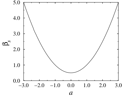
Fig. 12. Surface magnetization exponent \beta_s for the TM2 sequence with \kappa = 1/2 . The transition is always second-order and the critical behaviour is governed by a^2 .
