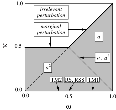
Fig. 1. Relevance-irrelevance of aperiodic extended surface perturbations in the Ising quantum chain. The perturbation is relevant in the shaded region. To first order in the amplitude a , the perturbation is relevant only below the first diagonal. Below the second diagonal and the line \kappa = 1/2 the second-order term is relevant and dominates the first-order one. On the marginal border line, the magnetization exponent is a function of a above \omega = 1/2 , of a^2 below, and involves both terms at \omega = 1/2 . The values of \omega for the aperiodic sequences used in the numerical FSS study are indicated.
