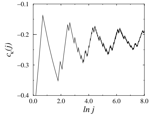
Fig. 8. Amplitude c_\kappa(j) as a function of \ln j for the TM1 sequence with \kappa = \omega . Asymptotically c_\kappa(j) converges towards the effective amplitude \bar{c} indicated on the left axis.
